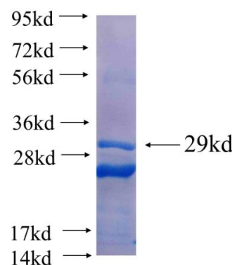
Recombinant human MFI2 SDS-PAGE
