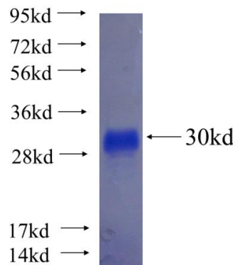
Recombinant human IGFBP1 SDS-PAGE
