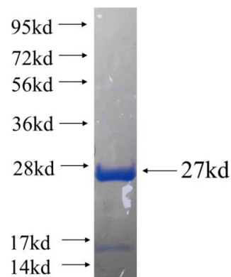
Recombinant human DHFR SDS-PAGE
