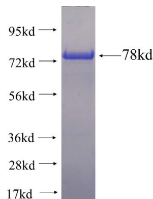
Recombinant human COPS2 SDS-PAGE
