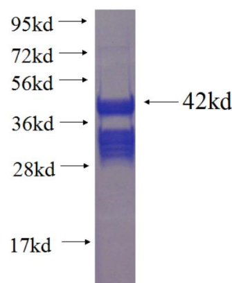
Recombinant human CHCHD2 SDS-PAGE
