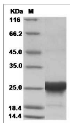
Human RAB31 / Rab22B Protein (His Tag) SDS-PAGE
